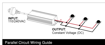
Parallel Circuit Wiring Guide
