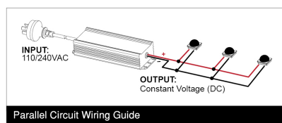
Diagram is a guide only. Wire colours and polarity may change depending on fixture and country.
